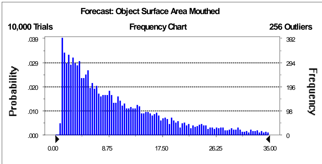
Figure B-1: Monte Carlo Simulation for Object Surface Area Mouthed ( \text{cm}^2 ) Assuming an Exponential Distribution (Minimum= 1 \text{ cm}^2 , Mean= 10 \text{ cm}^2 , Maximim= 50 \text{ cm}^2 )
